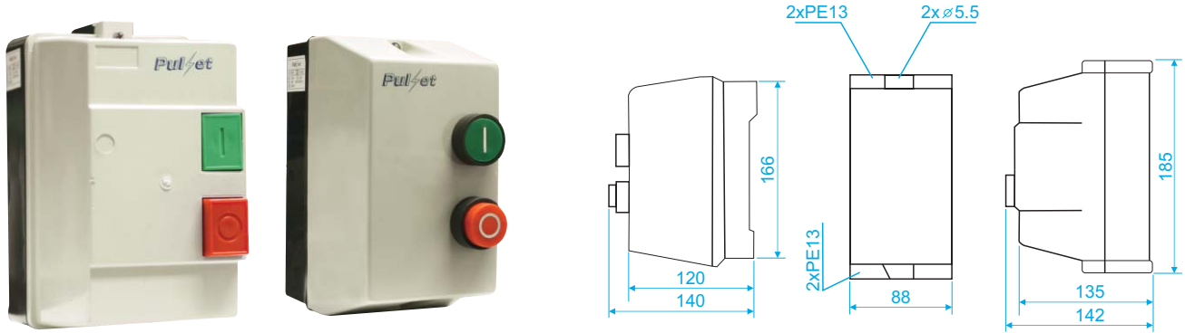
Dimensions in millimetres.
